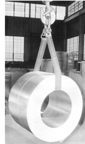
Type 2 Sling application
