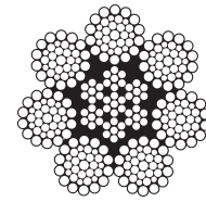
6 x 36 Warrington-Seale IWRC
